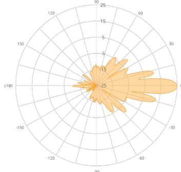
N5-X25 (25 dBi)
