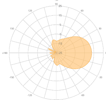
N5-X12 (12 dBi)
